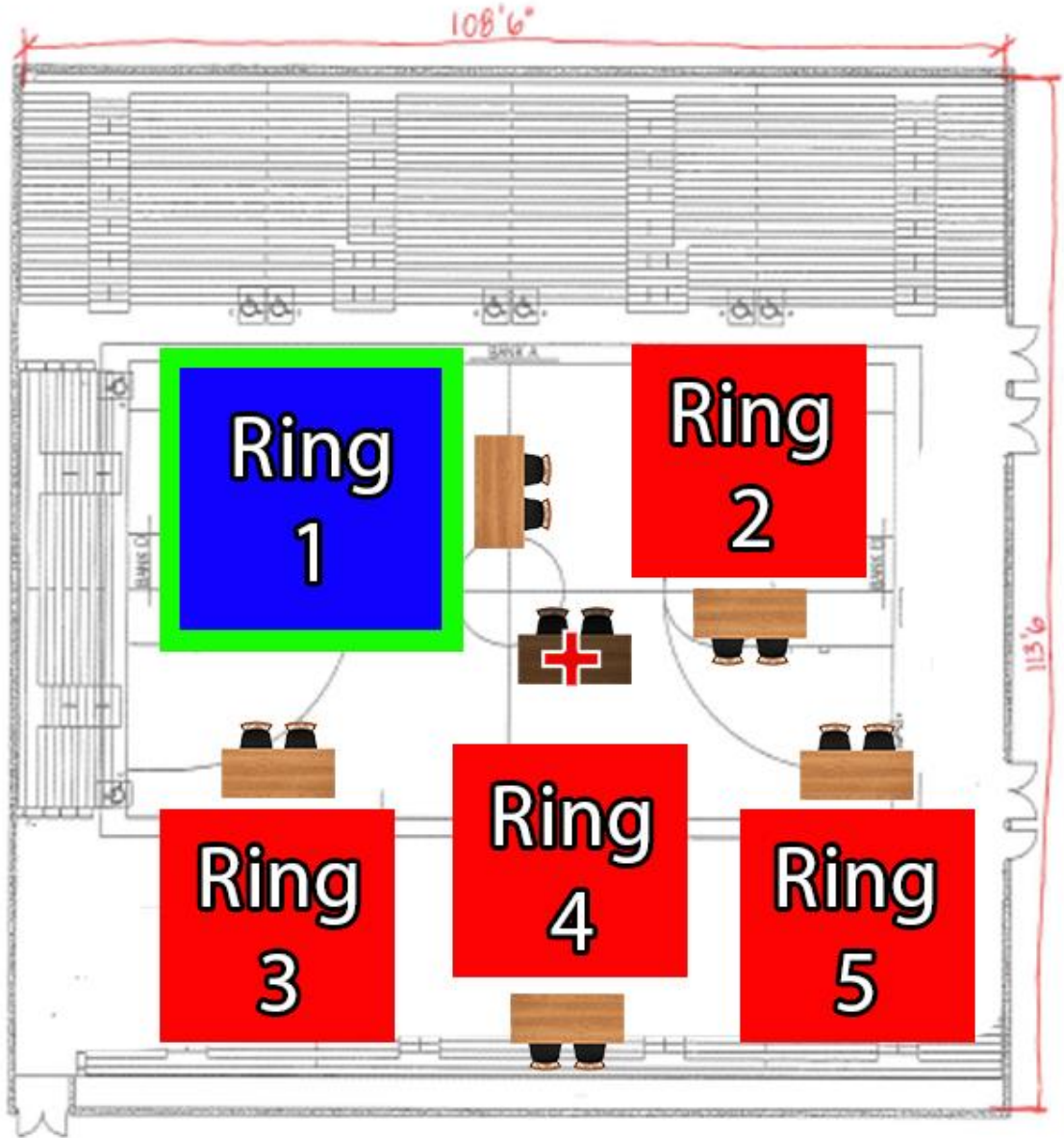
KEY PLAN 1/16" = 1'-0"
